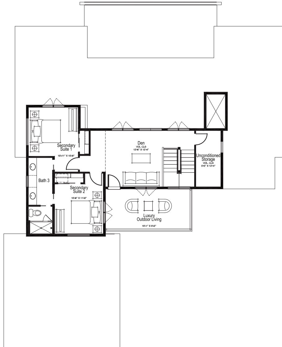
LOWER LEVEL FLOOR PLAN
