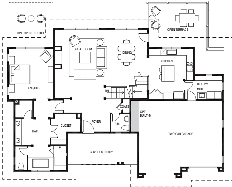
MAIN LEVEL
